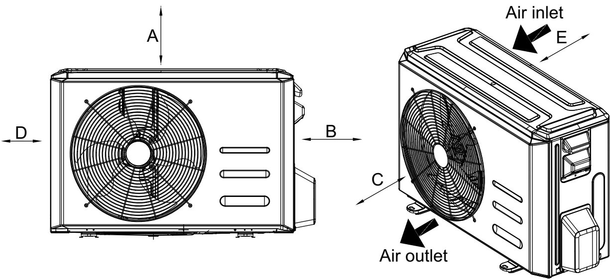
Fig. 6 — Clearances
